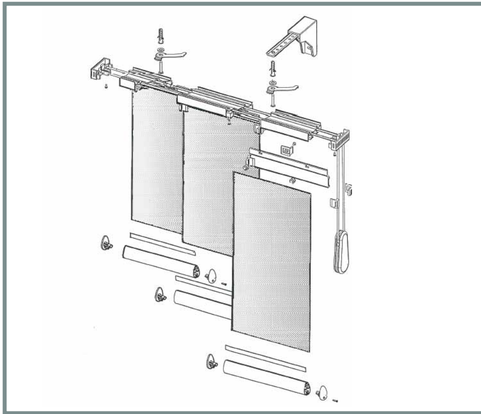
Linea Sliding Panel Track System Exploded view
