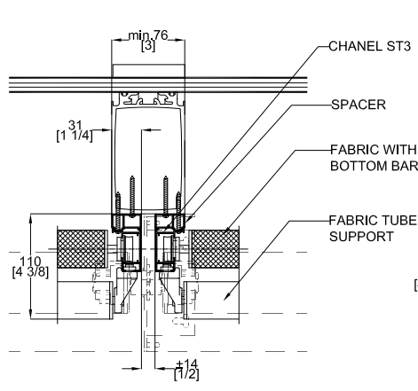
A2 INTERMEDIATE BRACKET TYPICAL INSTALLATION
