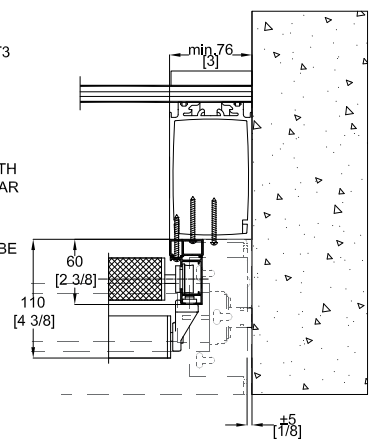
A3 MOTOR SIDE BRACKET TYPICAL INSTALLATION
