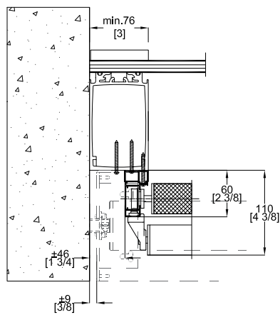
A1 IDLE SIDE BRACKET TYPICAL INSTALLATION
