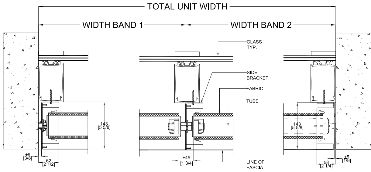
A1 IDLE SIDE BRACKET TYPICAL INSTALLATION
