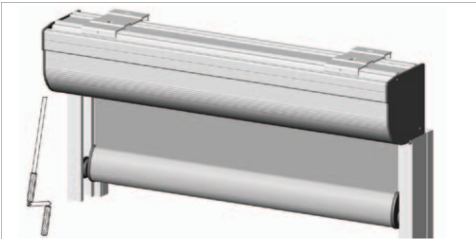
Tekno® Crank with Cassette 125 and Channels Type 3
