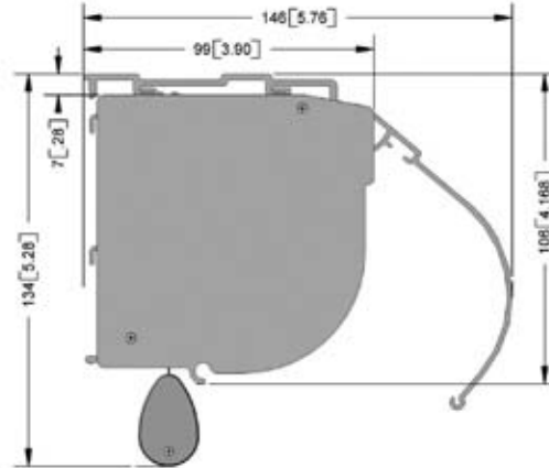
CASSETTE 70
