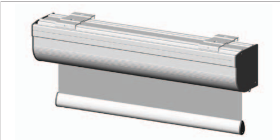
Tekno® Elektra 120V/AC With Cassette 95/125 — 400, 500 — 500 RTS
