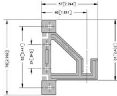
BRACKET TR
