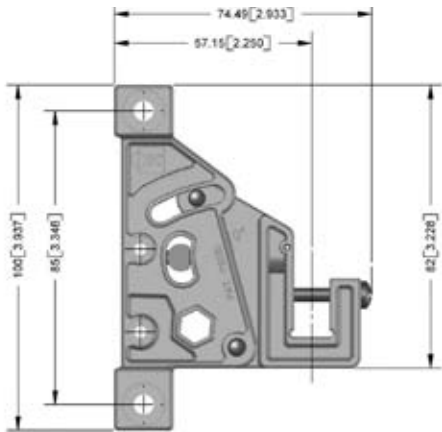
BRACKET HP
