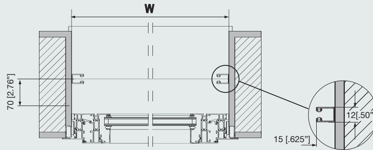
VP90 GTM (Optional Guide Cable)
