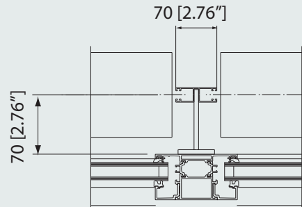
T470 INTERMEDIATE GUIDING TRACK (with TANDEM SYSTEM)
