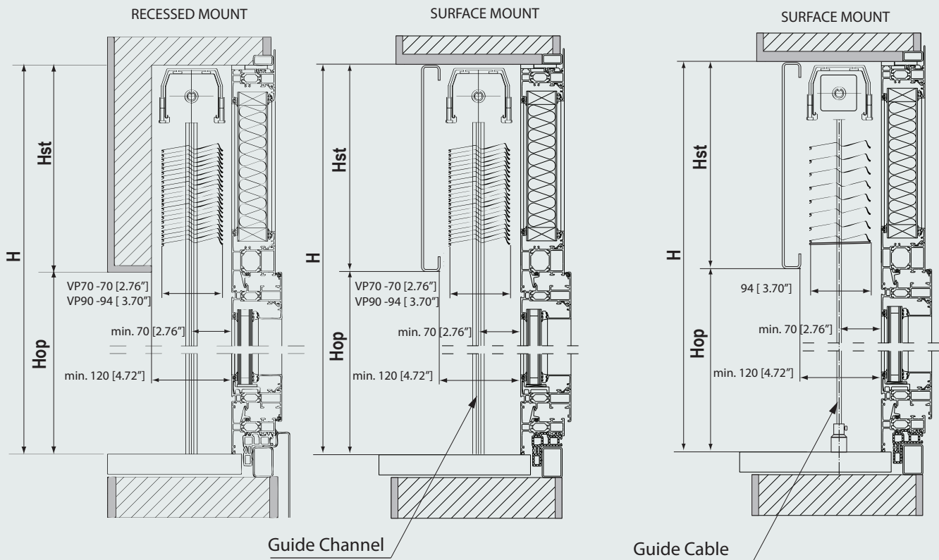
VP90 GTM (Optional Guide Cable)
