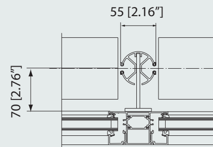
C550 INTERMEDIATE GUIDING TRACK (with TANDEM SYSTEM)
