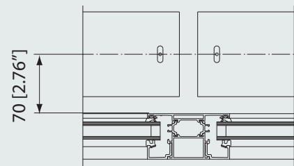
C550 INTERMEDIATE GUIDING TRACK (with TANDEM SYSTEM)
