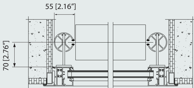
C550 SIDE GUIDING TRACKS (with SINGLE UNIT)
