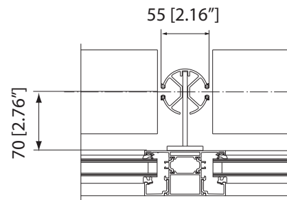
C550 INTERMEDIATE GUIDING TRACK (with TANDEM SYSTEM)
