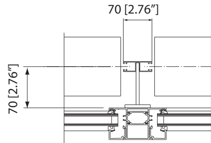
T470 INTERMEDIATE GUIDING TRACK (with TANDEM SYSTEM)
