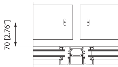
C550 INTERMEDIATE GUIDING TRACK (with TANDEM SYSTEM)
