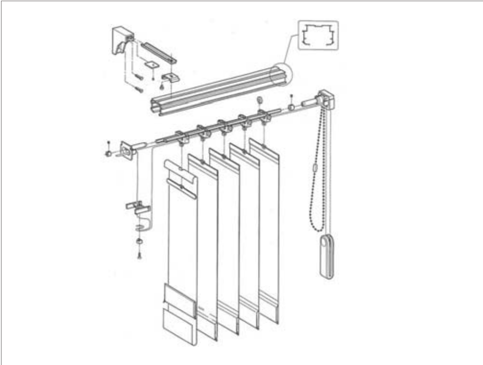
Solar Vertika Blinds Exploded view
